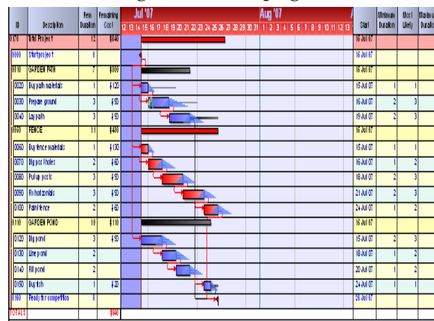
Fig. 8. Simulation program.
